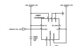
Barometer Sensor
