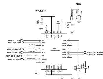
Audio amp
